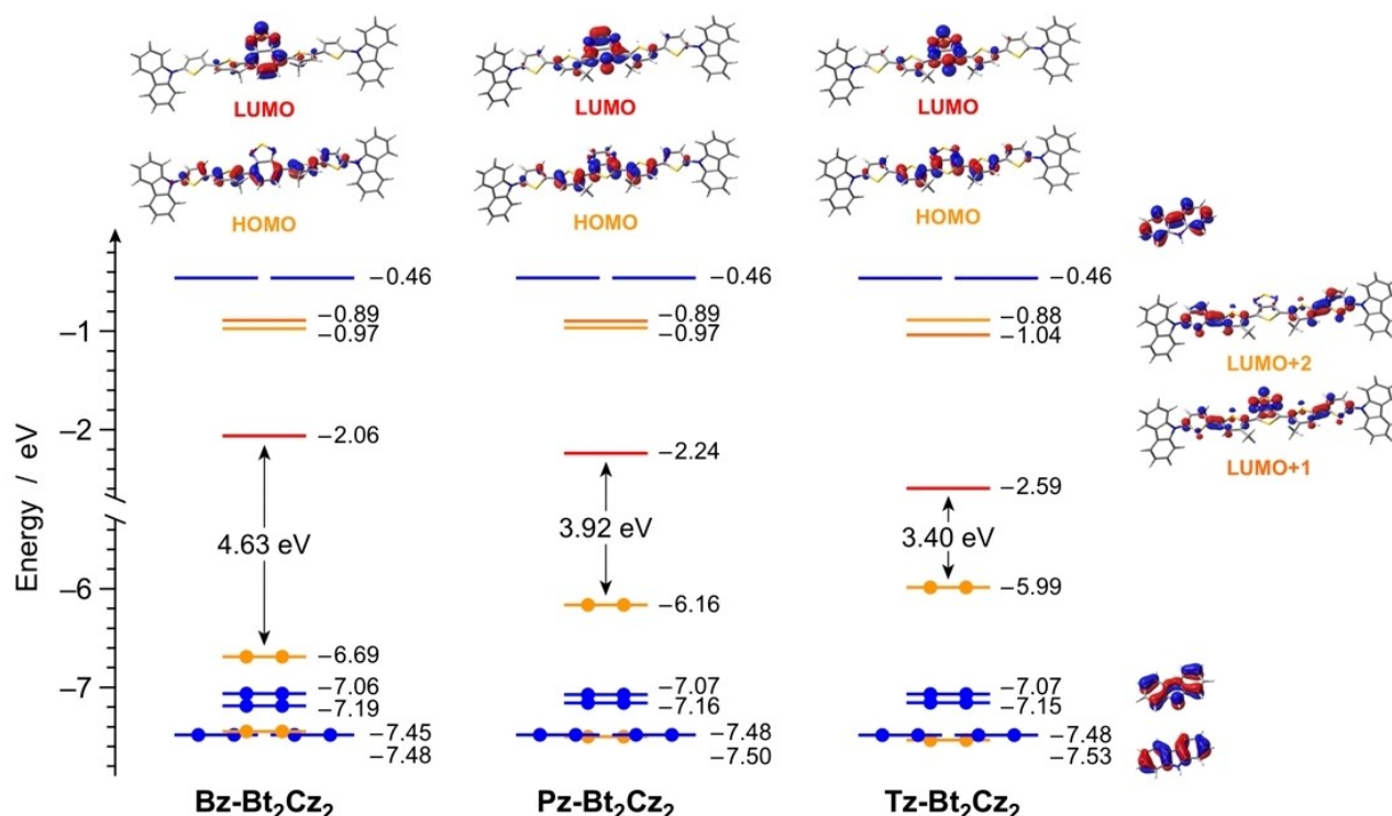
Figure 1. Energy diagram showing the energy values of the frontier Kohn-Sham molecular orbitals of Bz–Bt 2 Cz 2 , Pz–Bt 2 Cz 2 and Tz–Bt 2 Cz 2 in dichloromethane. For relevant orbitals, the corresponding isosurfaces are also displayed for clarity (isovalue = 0.04 e 1/2 bohr -3/2 ). Orbitals with similar topology are plotted with the same color for easier comparison (e.g., carbazole-based orbitals are reported in blue and displayed in a compact way using pristine 9H-carbazole as a model compound).
